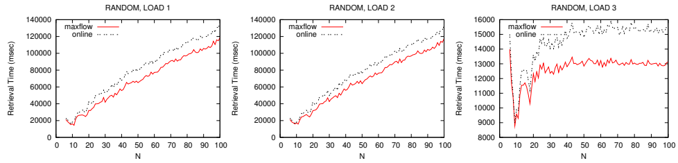
Figure 6: Max-flow vs. Online, Arbitrary, Random
