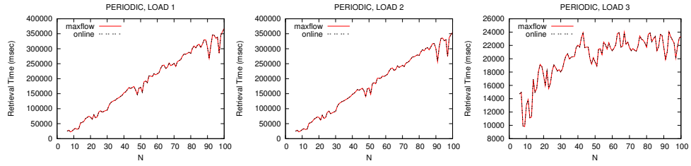
Figure 5: Max-flow vs. Online, Arbitrary, Periodic
