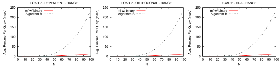
Figure 27: Running time, Range Queries
