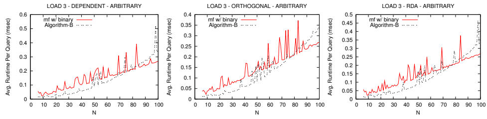
Figure 28: Running time, Arbitrary Queries
