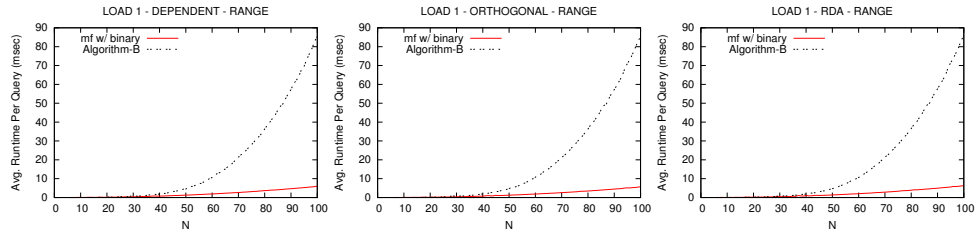
Figure 24: Running time, Range Queries
