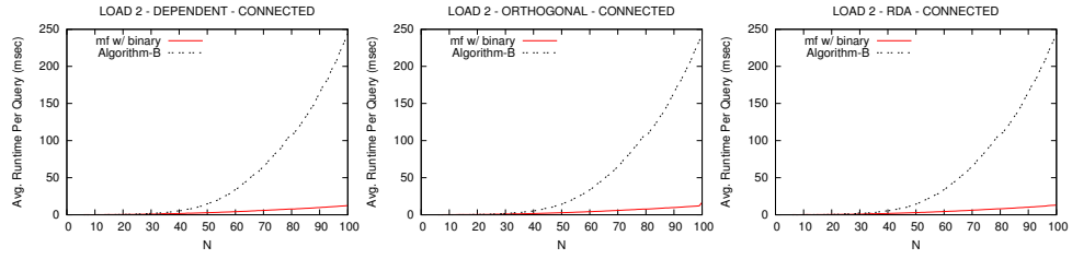
Figure 26: Running time, Connected Queries
