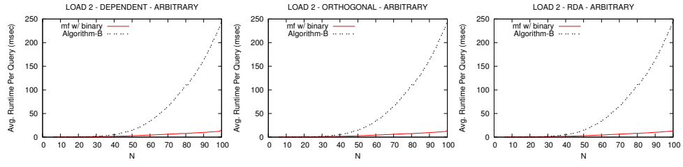
Figure 25: Running time, Arbitrary Queries
