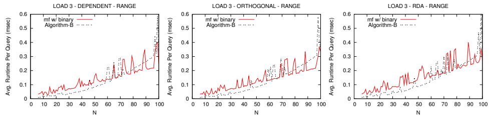
Figure 30: Running time, Range Queries
