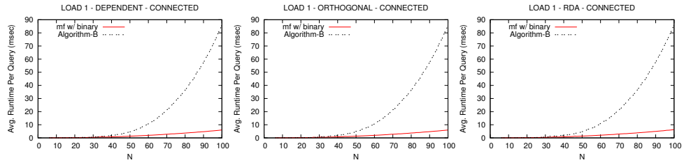
Figure 23: Running time, Connected Queries
