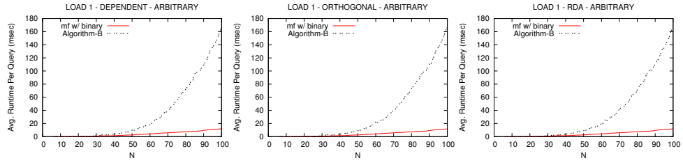
Figure 22: Running time, Arbitrary Queries
